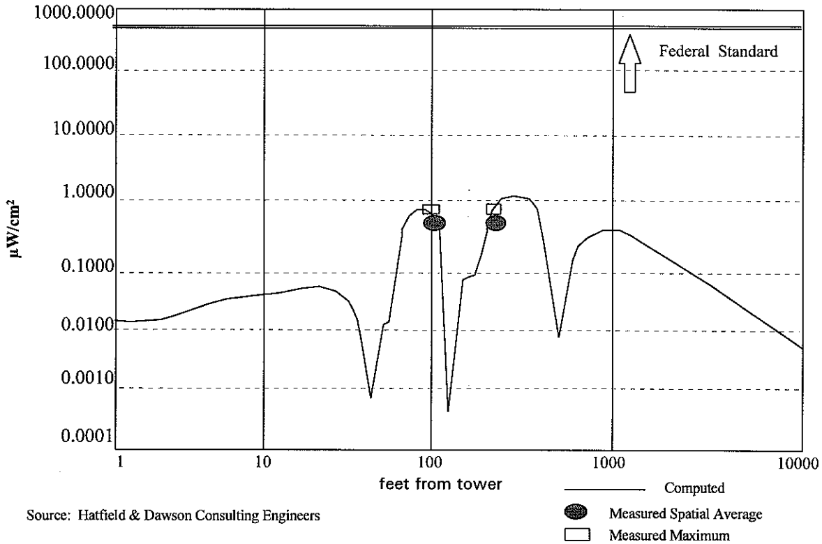
FIGURE 1. COMPUTED & MEASURED POWER DENSITY - 1800 Watts ERP
