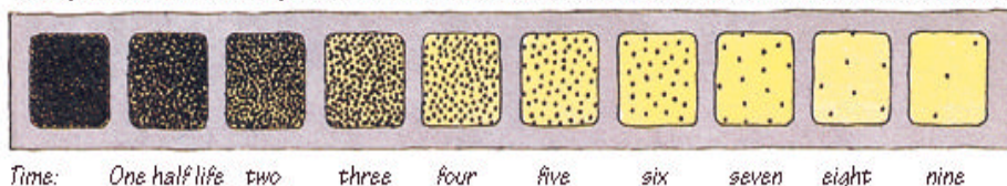
Decay rate of radioactivity: After ten half lives, the level of radiation is reduced to one thousandth
