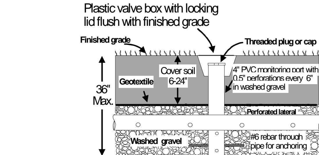
Figure 4. Typical Monitoring Port Detail
