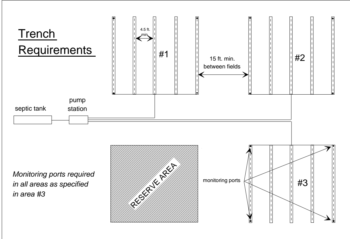
Figure 1: Drainfield Area Requirements
