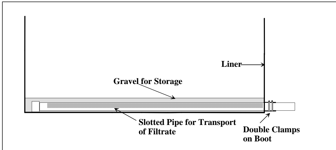
Figure 4 - Typical Cross-section of a Recirculating Gravel Filter Underdrain
