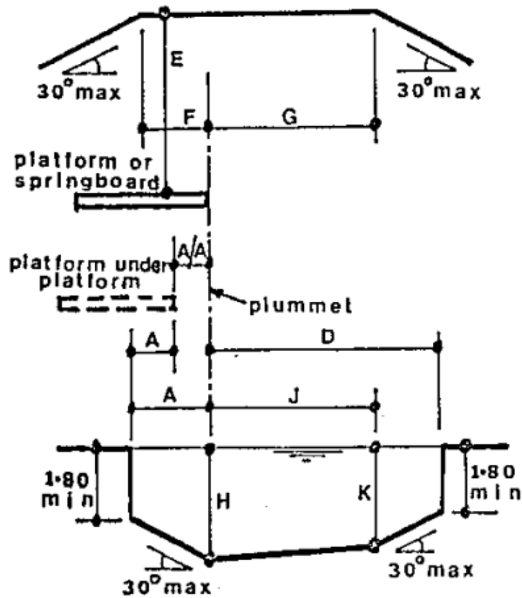
FIGURE 2 Minimum dimensions for pools with boards or platforms at a height of one-half meter or more.
