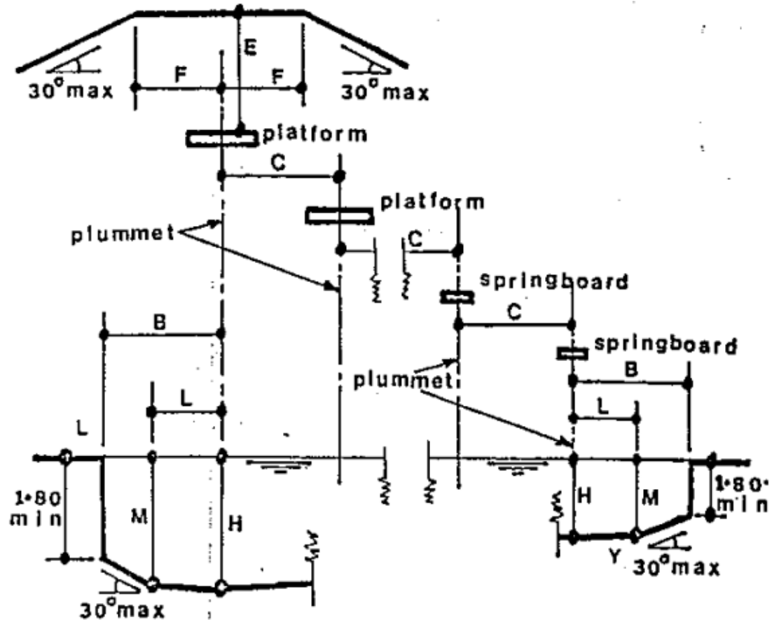
FIGURE 2 Minimum dimensions for pools with boards or platforms at a height of one-half meter or more.
