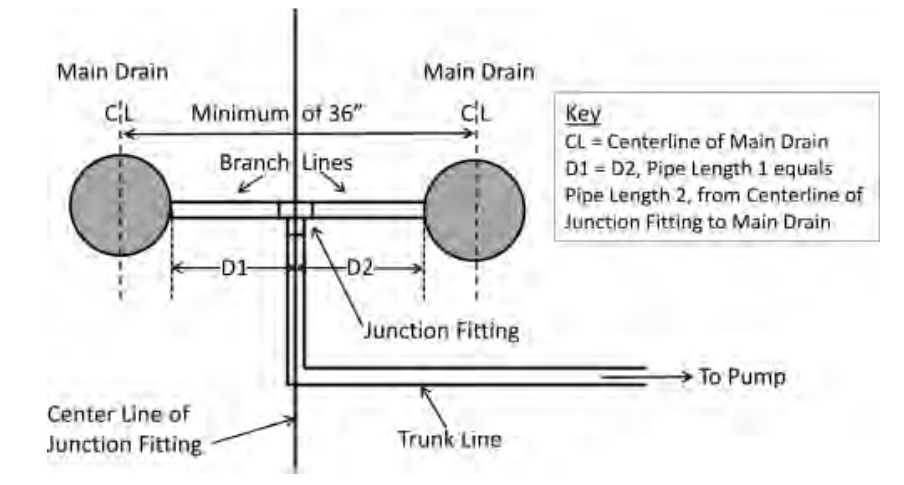
FIGURE 3: Main Drain Branch Line Piping Detail.
