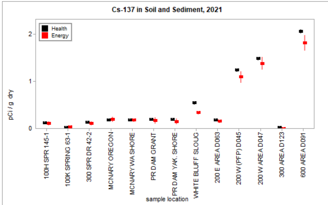
Figure 3.4.2 – Split Cs-137 Concentrations in Soil and Sediment
