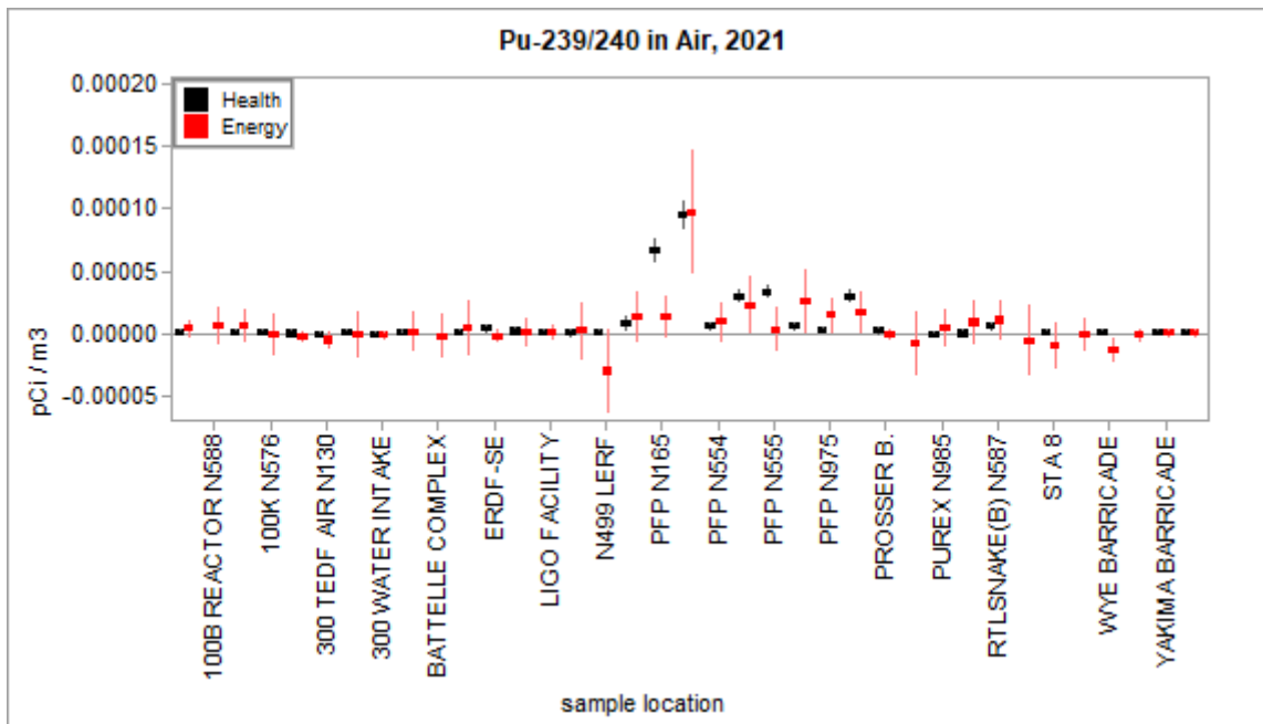
Figure 3.1.11 – Health and Energy Pu-239/240 Concentrations in Air All Data
