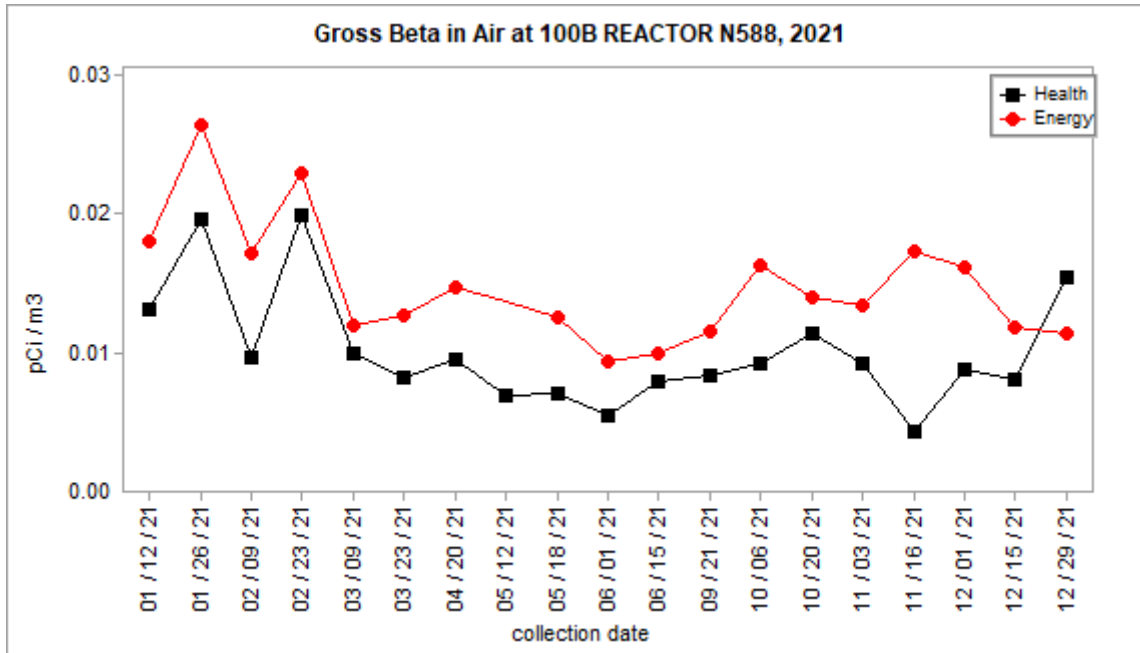
Figure 3.1.4 – Health and Energy Gross Beta Concentrations in Air at 100B Reactor
