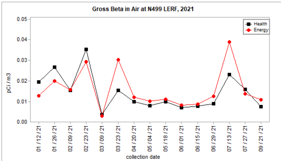
Figure 3.1.5 – Health and Energy Gross Beta Concentrations in Air at Liquid Effluent Retention Facility (LERF)
