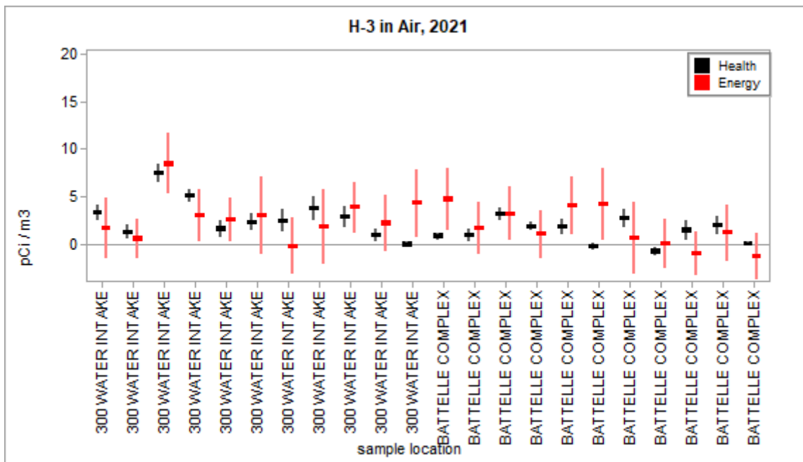
Figure 3.1.7 – Health and Energy H-3 Concentrations in Air
