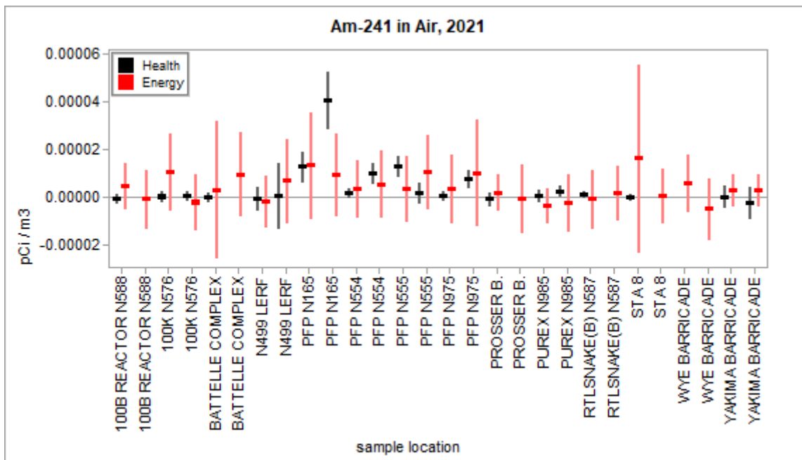
Figure 3.1.9 – Health and Energy Am-241 Concentrations in Air All Data
