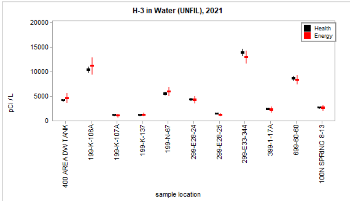
Figure 3.2.9 – Health and Energy H-3 Concentrations in Water Low-Range Data
