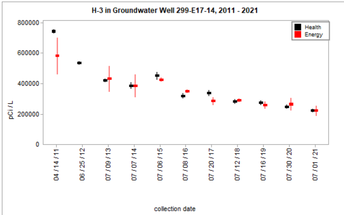
Figure 3.2.10 – Health and Energy H-3 Concentrations in Water at Groundwater Well 299-E17-14
