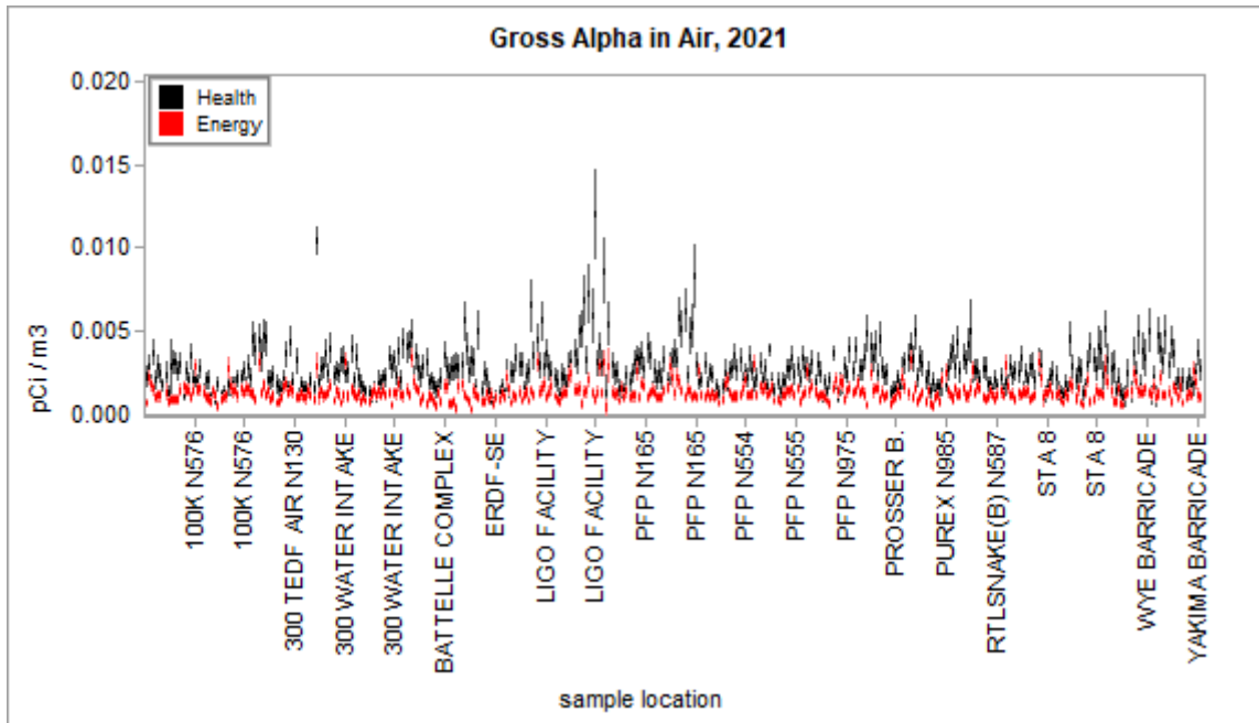
Figure 3.1.2 – Health and Energy Gross Alpha Concentrations in Air
