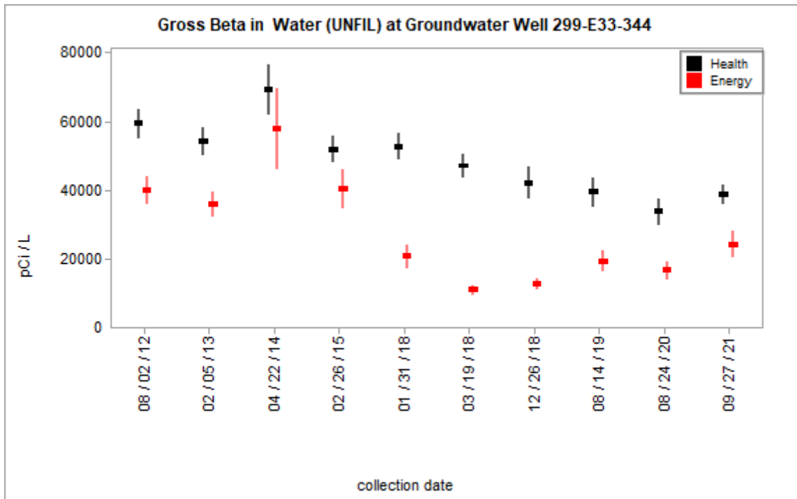
Figure 3.2.7 – Health and Energy Gross Beta Concentrations in Water at Groundwater Well 299-E33-344
