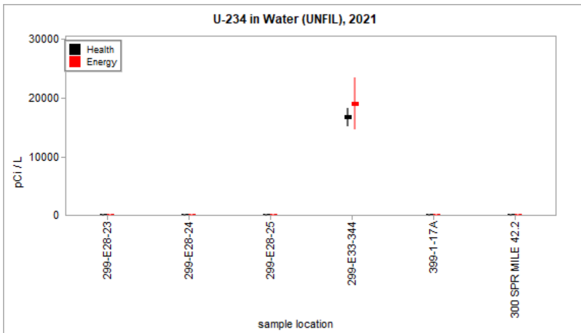
Figure 3.2.15 – Health and Energy U-234 Concentrations in Water All Data
