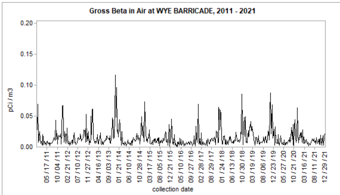
Figure 3.1.17 – Gross Beta in Air at Wye Barricade 2011 – 2021
