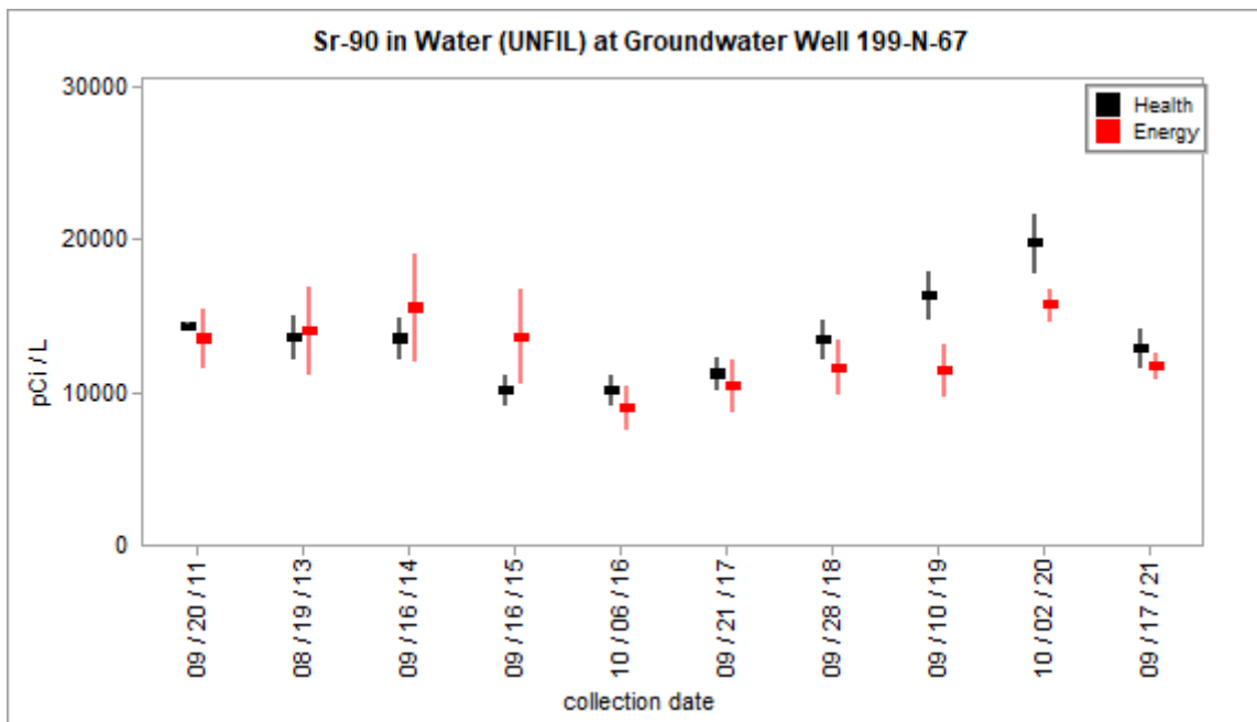
Figure 3.2.13 – Health and Energy Sr-90 Concentrations in Water at Groundwater Well 199-N-67
