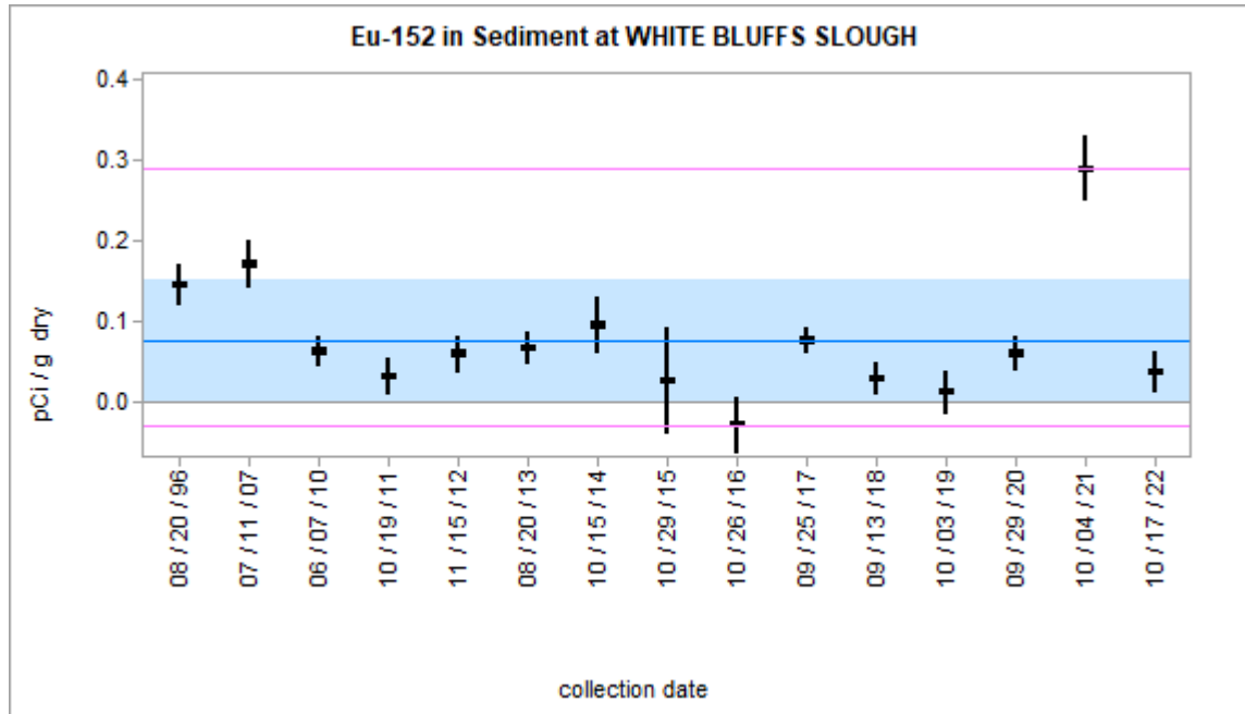
Figure 3.4.4 – Health Eu-152 Concentrations in Sediment at White Bluff
