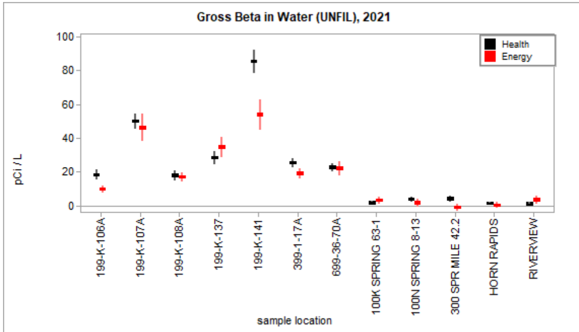
Figure 3.2.6 – Health and Energy Gross Beta Concentrations in Water Low-Range Data
