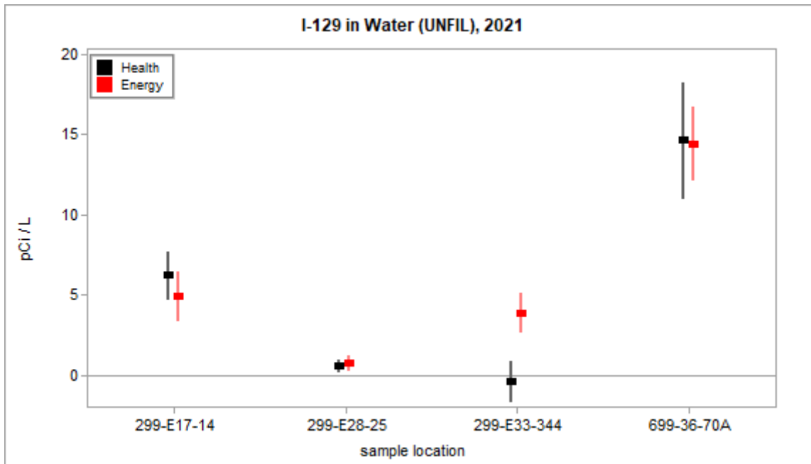
Figure 3.2.11 – Health and Energy I-129 Concentrations in Water
