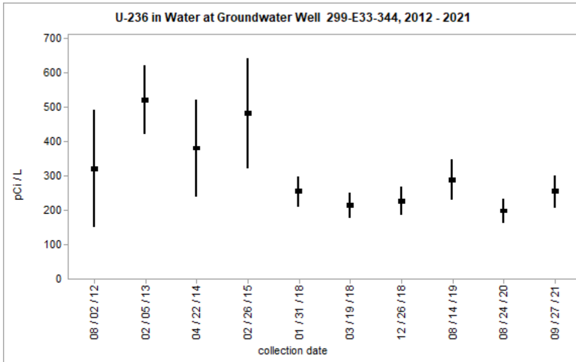
Figure 3.2.18 – Health U-236 Concentrations in Water at Groundwater Well 299-E33-344
