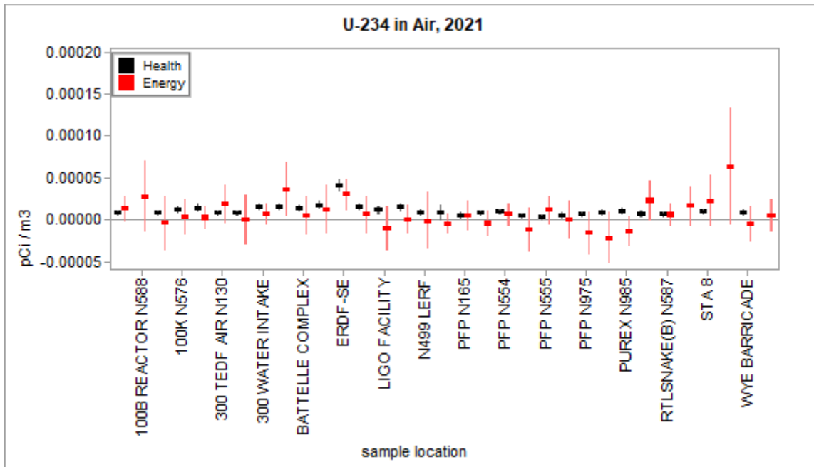
Figure 3.1.16 – Health and Energy U-234 Concentrations in Air
