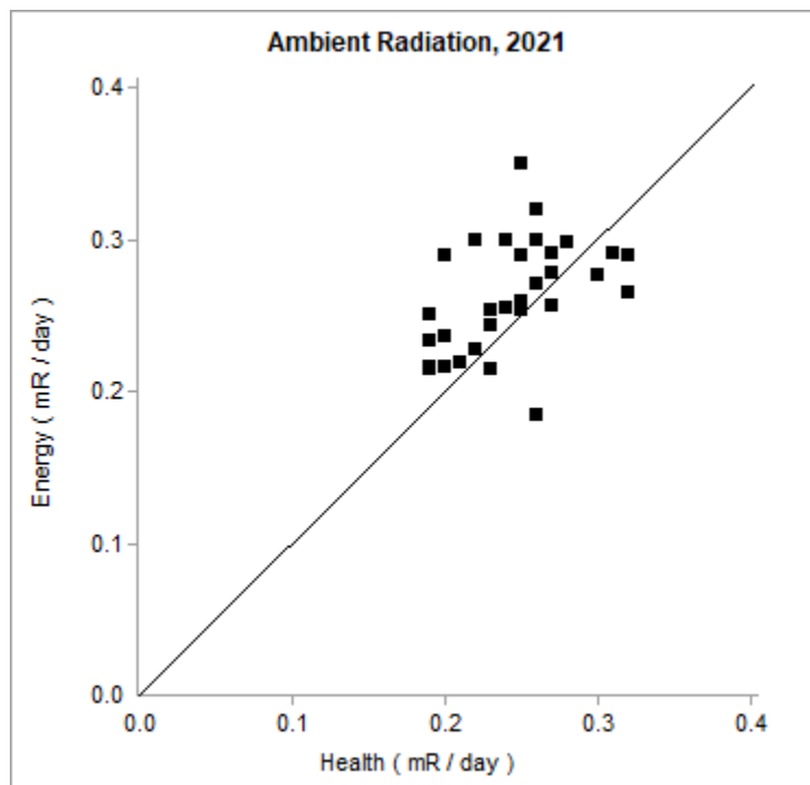
Figure 3.3.3 – Health and Energy Quarterly Ambient Radiation
