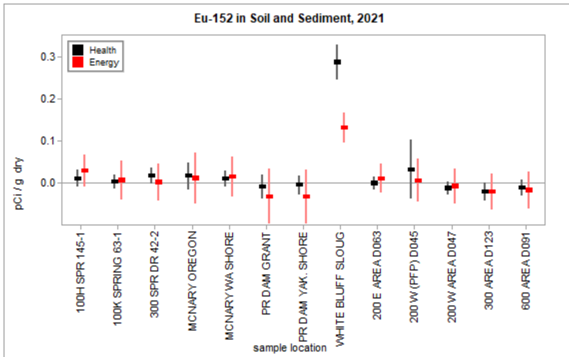
Figure 3.4.3 – Split Eu-152 Concentrations in Soil and Sediment
