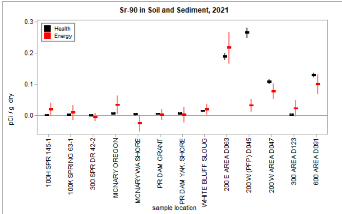
Figure 3.4.6 – Split Sr-90 Concentrations in Soil and Sediment
