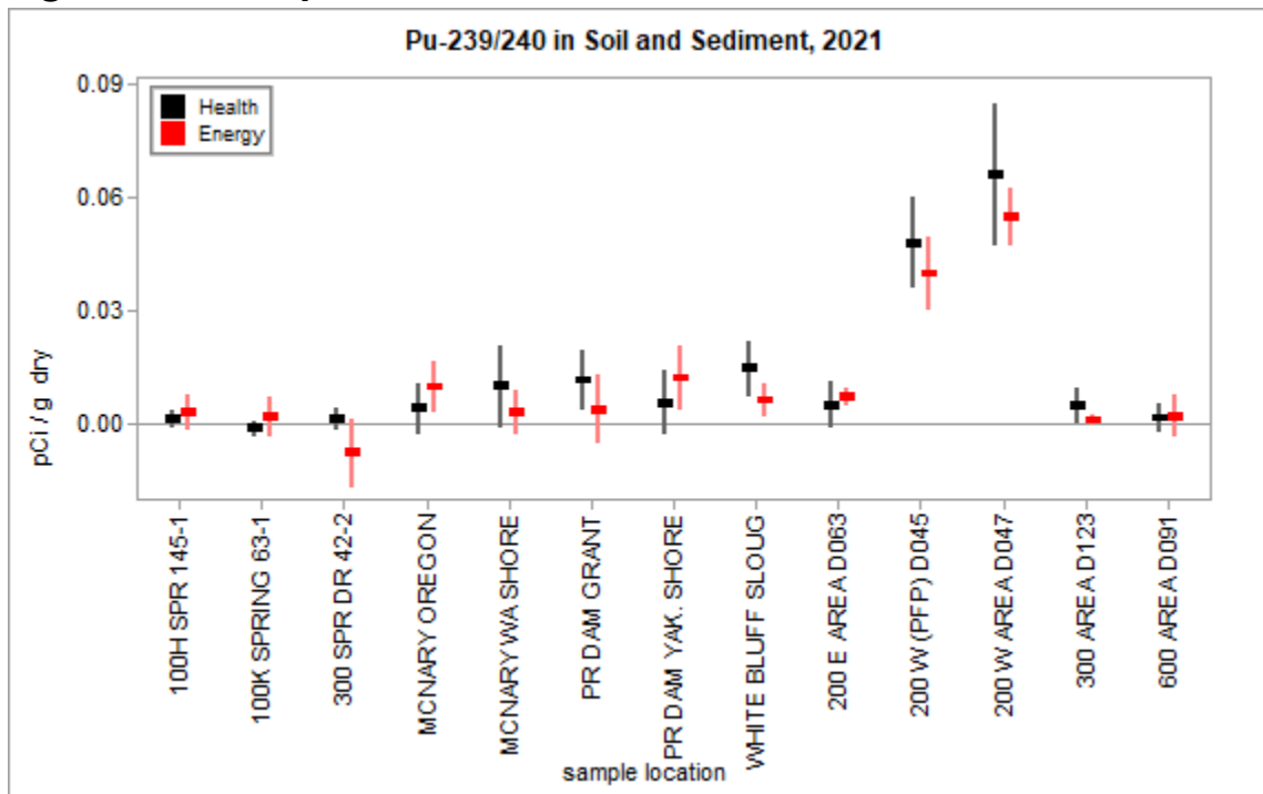
Figure 3.4.5 – Split Pu-239/240 Concentrations in Soil and Sediment
