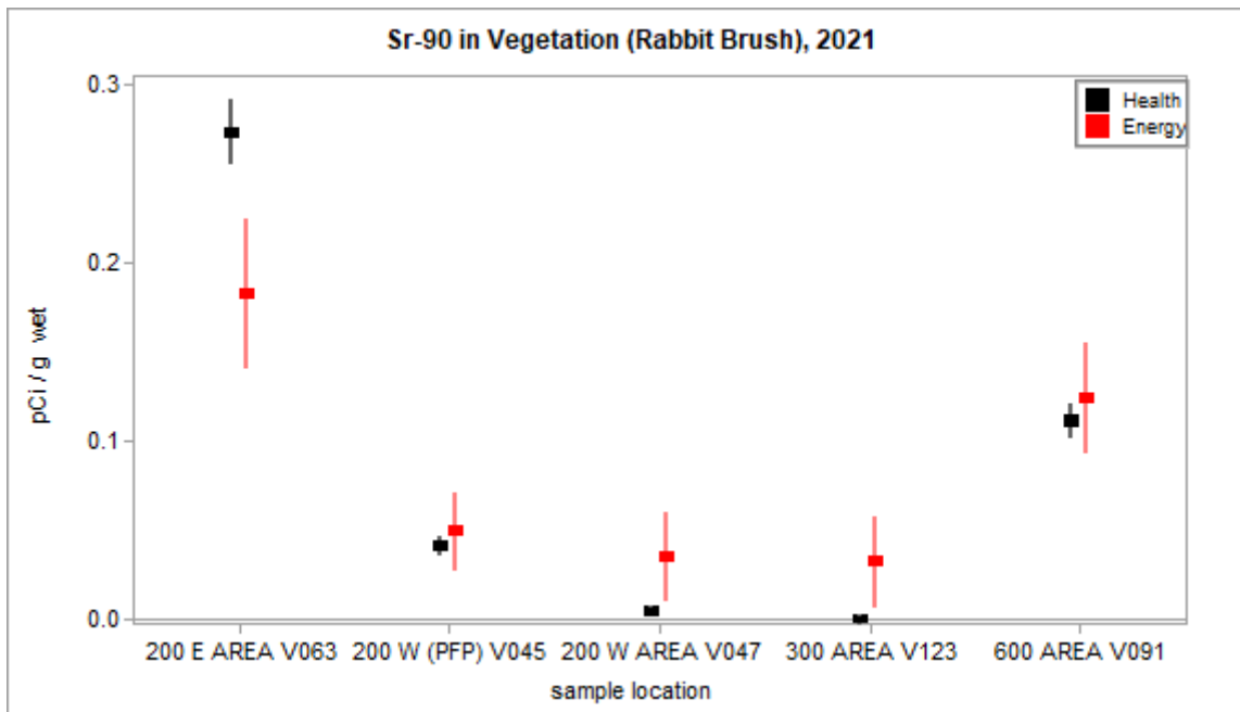
Figure 3.5.2 – Health and Energy Sr-90 Concentrations in Vegetation
