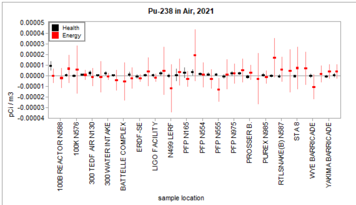
Figure 3.1.10 – Health and Energy Pu-238 Concentrations in Air
