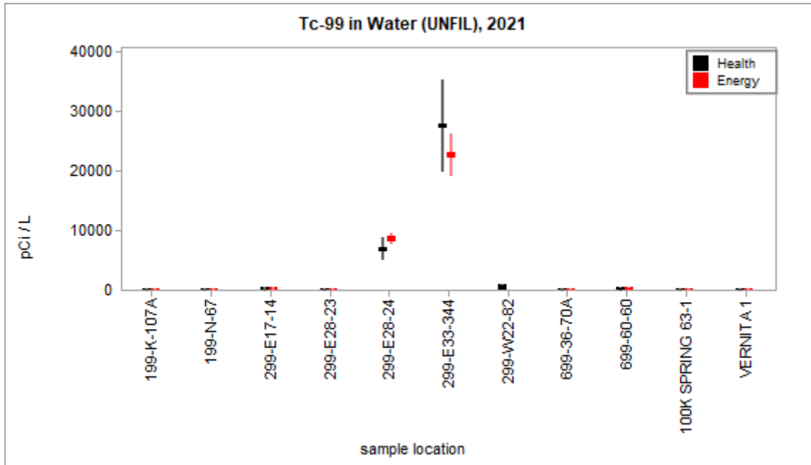
Figure 3.2.14 – Health and Energy Tc-99 Concentrations in Water
