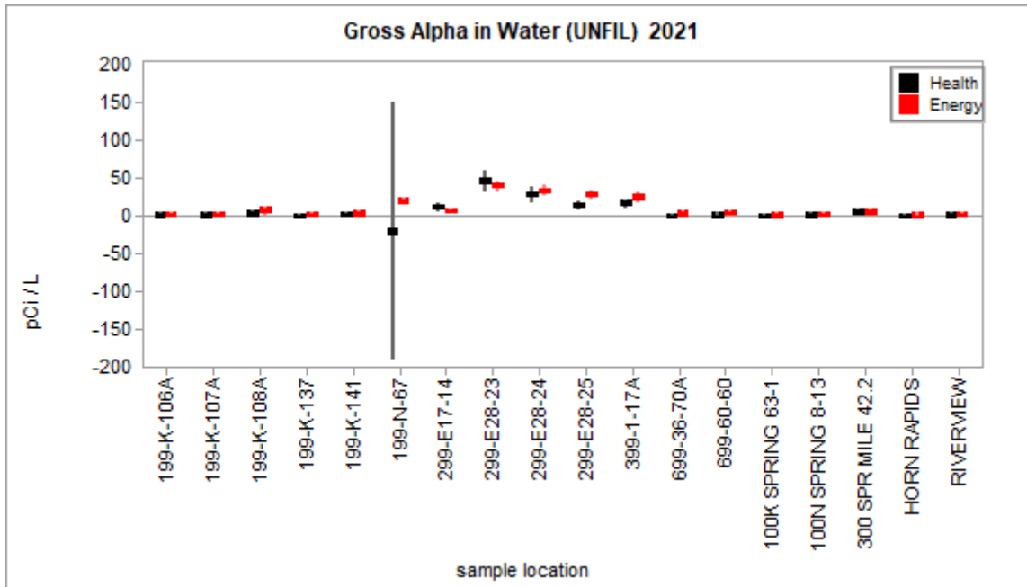
Figure 3.2.5 – Health and Energy Gross Alpha Concentrations in Water, Low-Range Data
