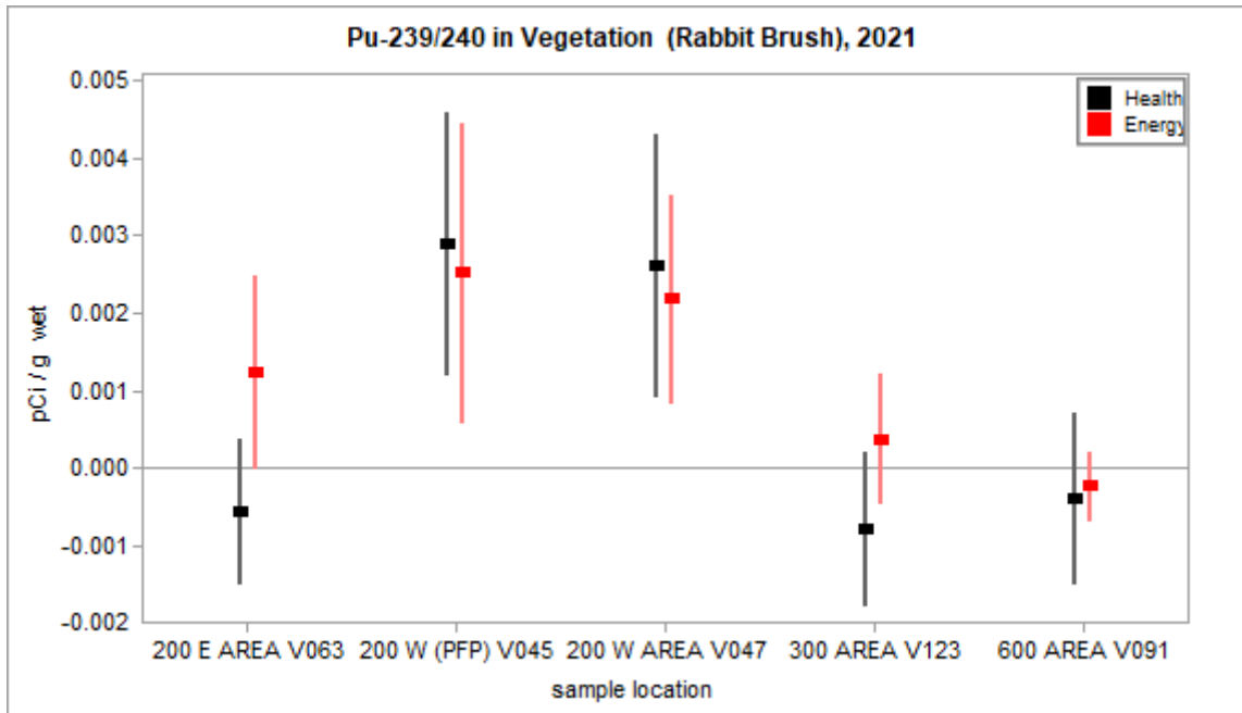
Figure 3.5.1 – Health and Energy Pu-239/240 Concentrations in Vegetation
