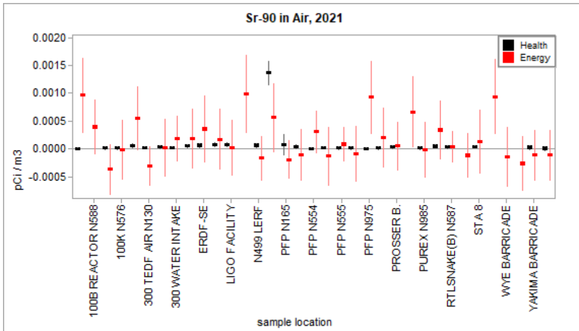
Figure 3.1.15 – Health and Energy Sr-90 Concentrations in Air
