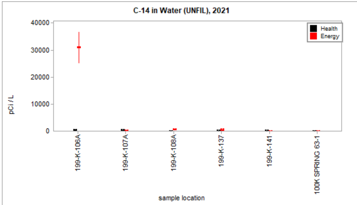
Figure 3.2.2 – Health and Energy C-14 Concentrations in Water All Data
