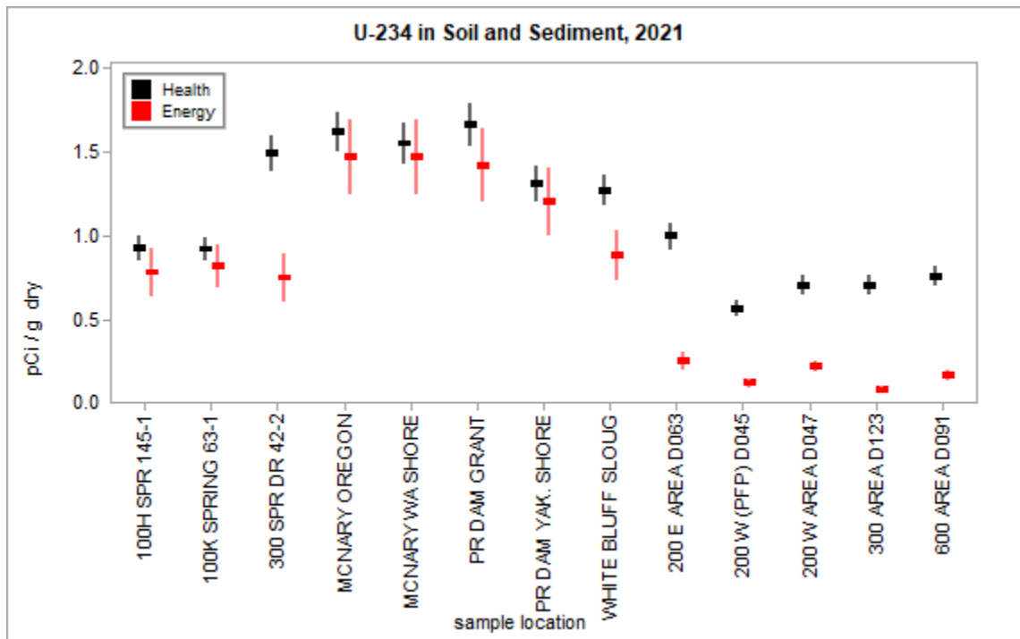
Figure 3.4.7 – Split U-234 Concentrations in Soil and Sediment
