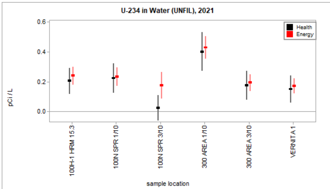
Figure 3.2.17 – Health and Energy U-234 Concentrations in Water Low-Range Data
