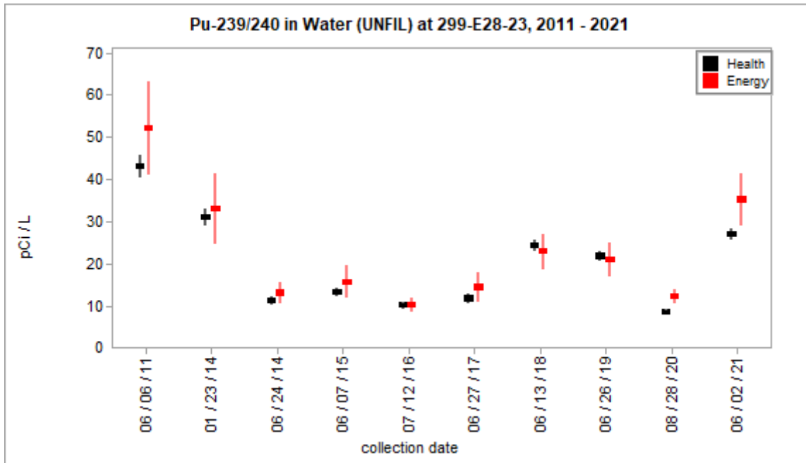
Figure 3.2.12 – Health and Energy Pu-239/240 Concentrations in Water at Groundwater Well 299-E28-23
