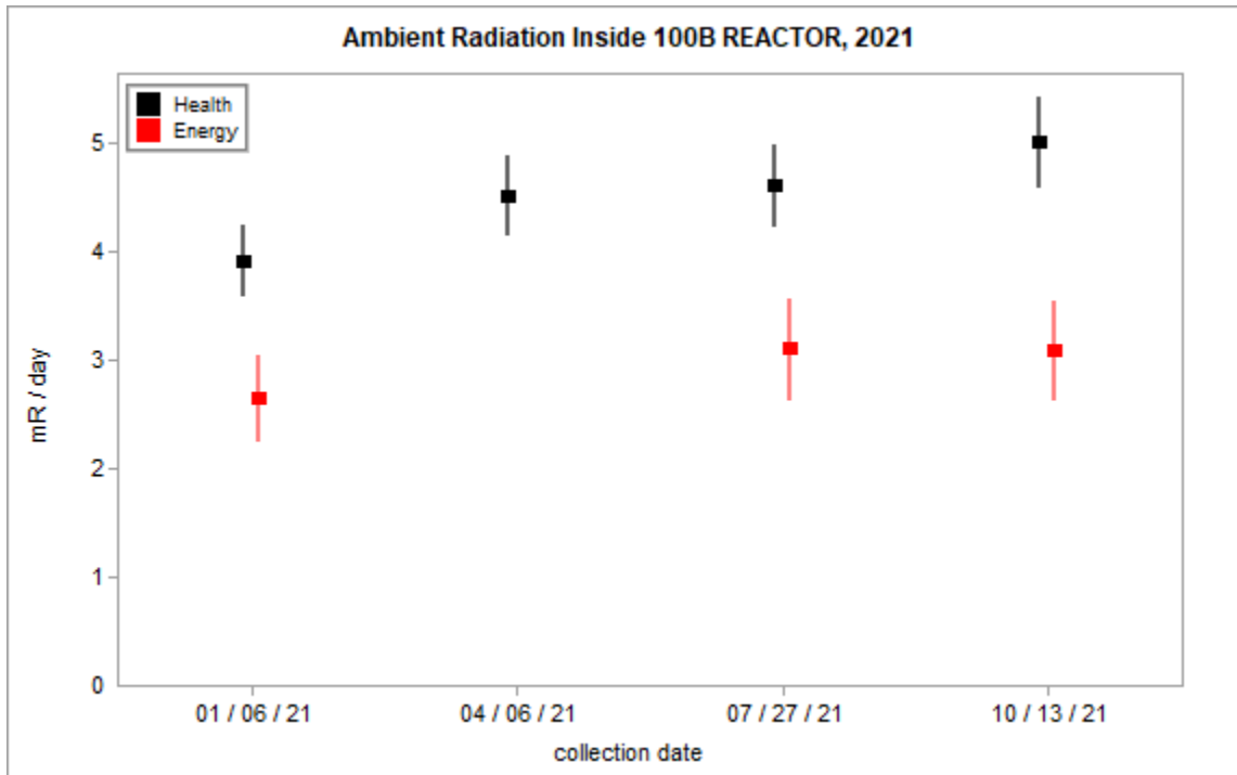
Figure 3.3.4 – Health and Energy Quarterly Ambient Radiation at 100B Reactor
